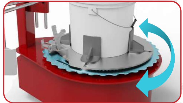
Rotate the wheel to adjust the width of the clamps for different sized containers
